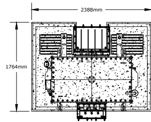
TRANSFORMER (TX) PLAN VIEW
